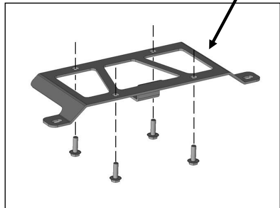
(Fig 21) Attach winch control to Relocation Bracket
