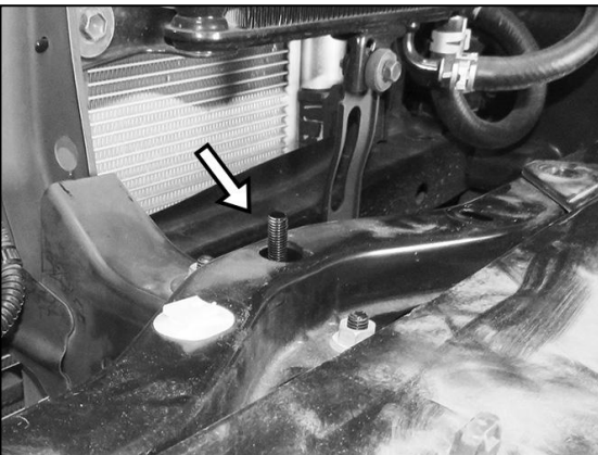
(Fig 22) Insert Bolt Plate into hole in top of crossmember (arrows)
