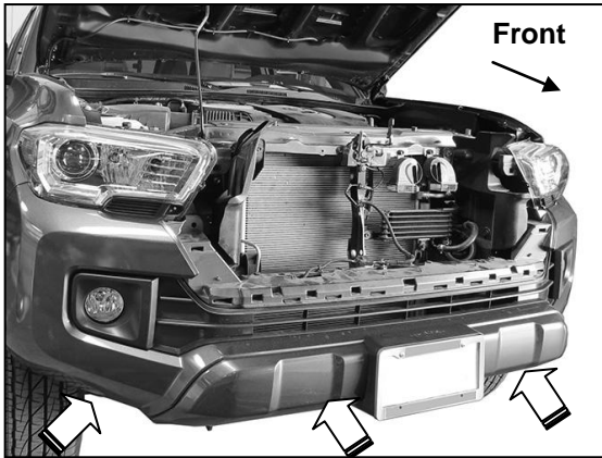
(Fig 3) Remove hardware attaching bottom of bumper to vehicle (arrows)
