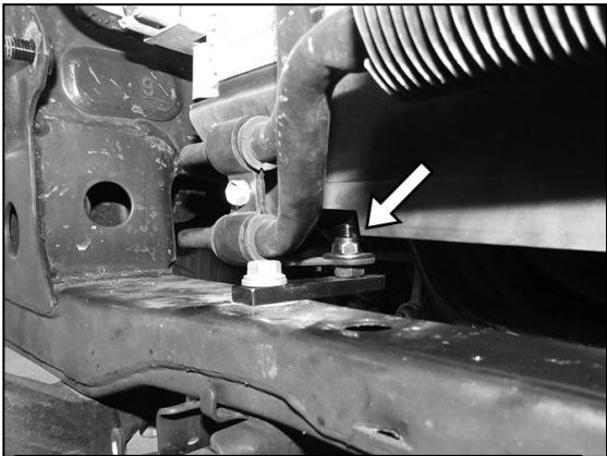
(Fig 15) Passenger/right side of cooler relocated towards the radiator (arrow)
