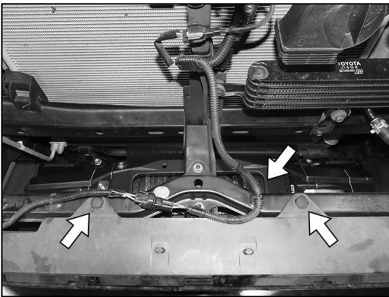
(Fig 20) Release clips and move wire harness. Remove (2) clips attaching top of bumper cover (arrows)
