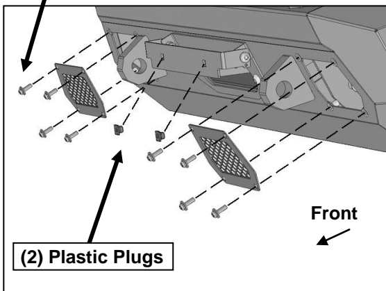
(Fig 30) Attach Mesh Fill Panels (driver/left side illustrated)
