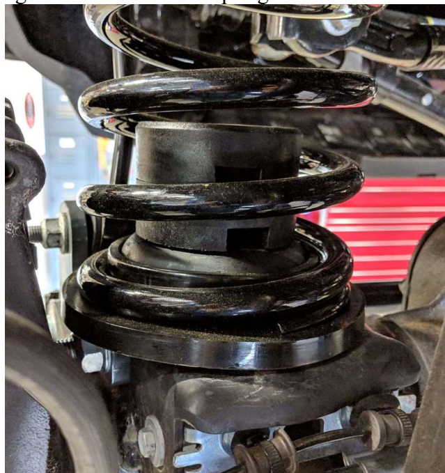
Figure 1. Correctly Installed Lower Spring Isolator
