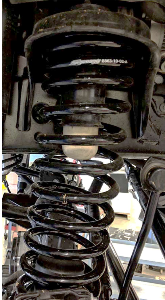
Figure 2. Correctly Installed Front Coil Spring
