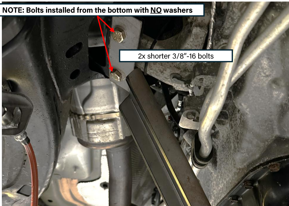
Figure 35: CAD and installation of passenger side motor mount bracket
