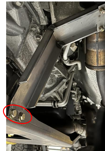
Figure 37: New skid plate installed at OEM 3.6L motor mount locations and skid plate connections
