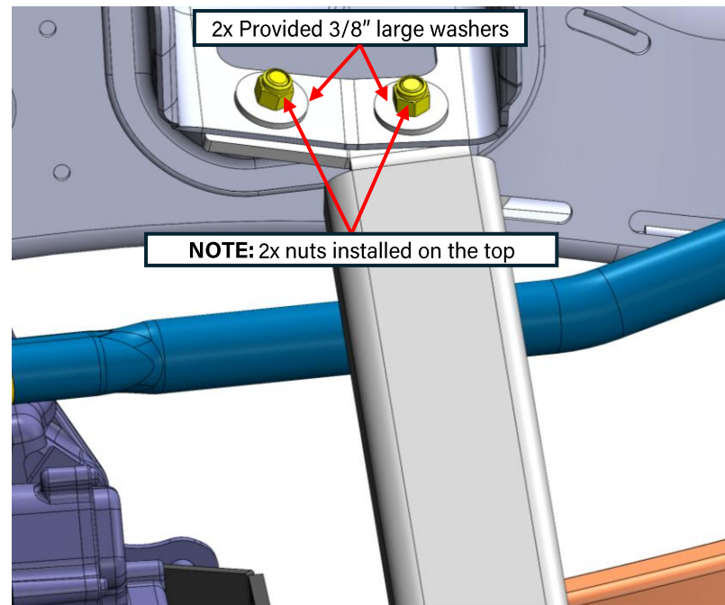
Figure 35: CAD and installation of passenger side motor mount bracket
