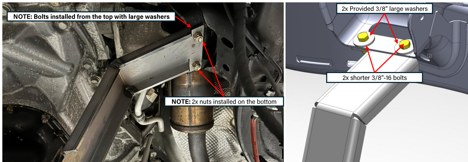
Figure 34: CAD and installation of driver-side motor mount bracket
