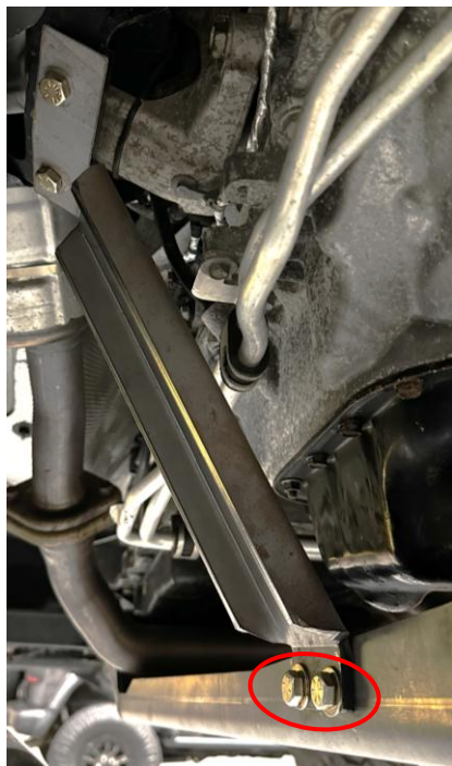
Figure 37: New skid plate installed at OEM 3.6L motor mount locations and skid plate connections
