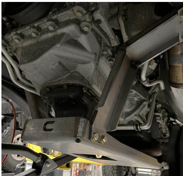
Figure 39: Engine skid plate fully installed
