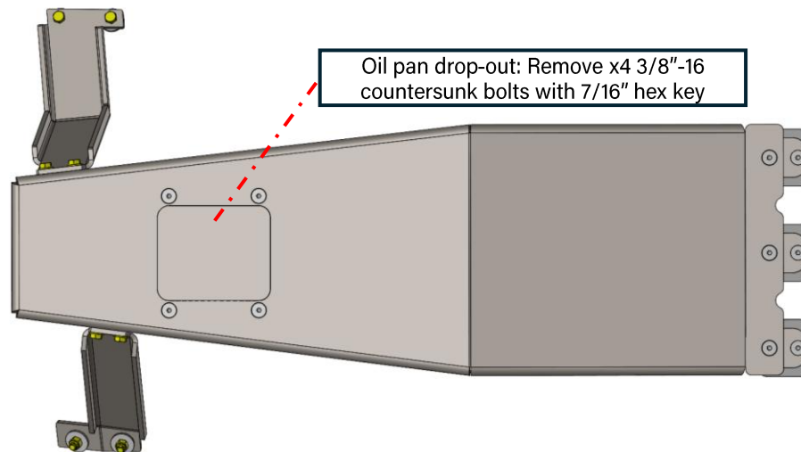
Figure 38: Oil pan drop-out for oil changes and service
